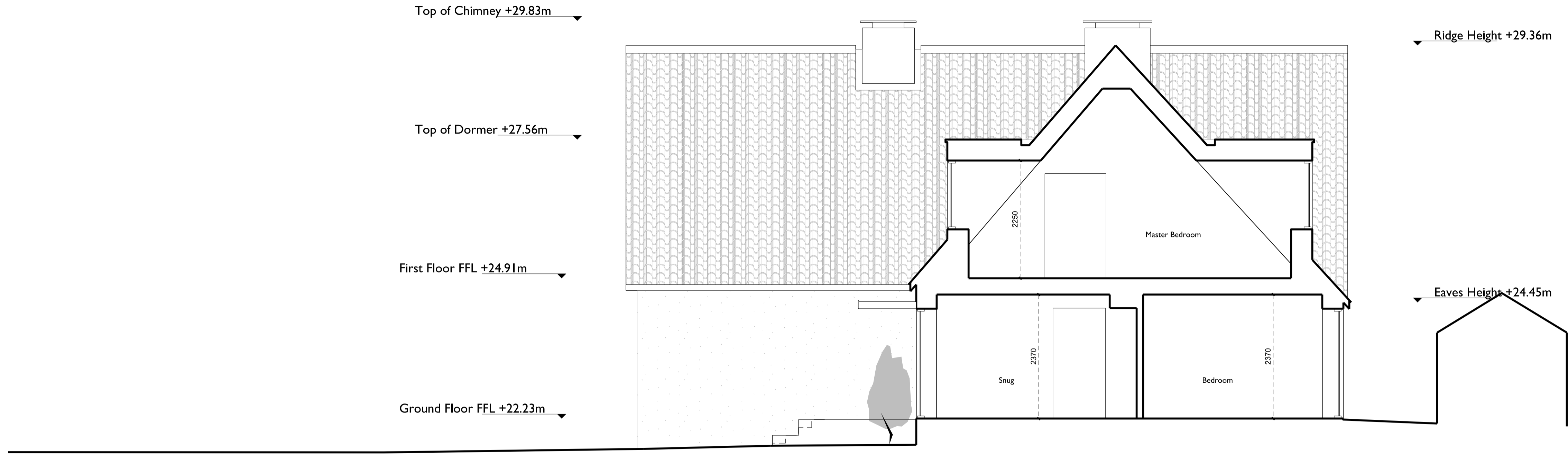
01 PROPOSED SECTION AA 1:50 @ A1 or 1:100 @ A3 16000
