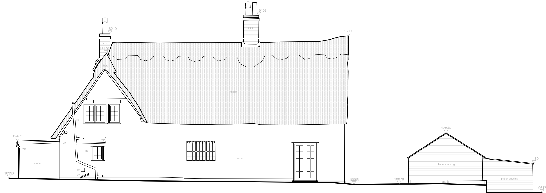
South Elevation
