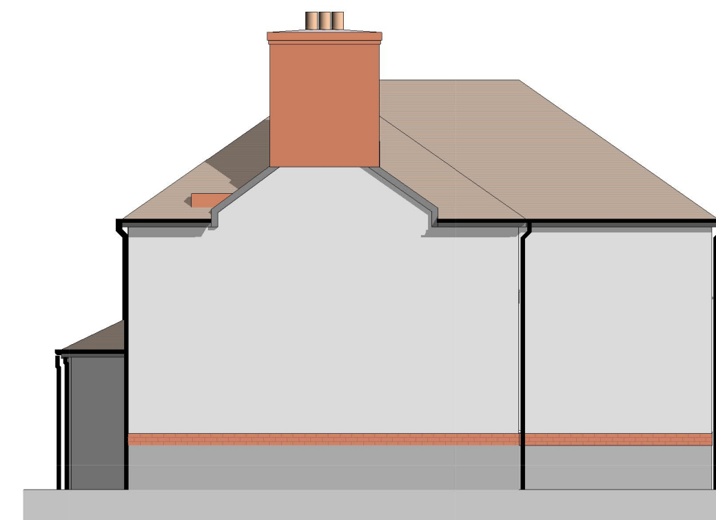
Right Side Elevation Type 3 1 : 100
