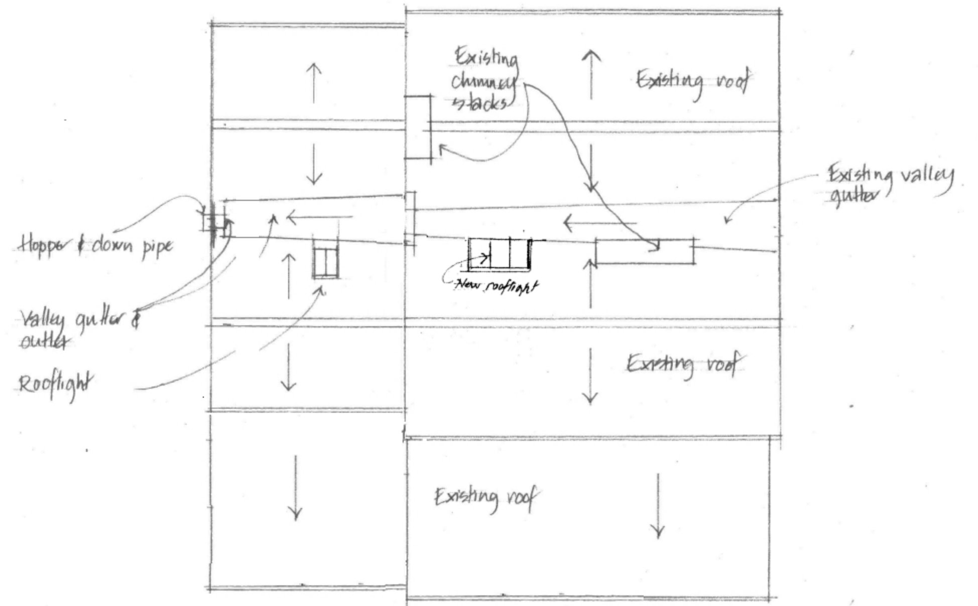
Roof Plan
