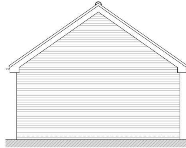
East Elevation
