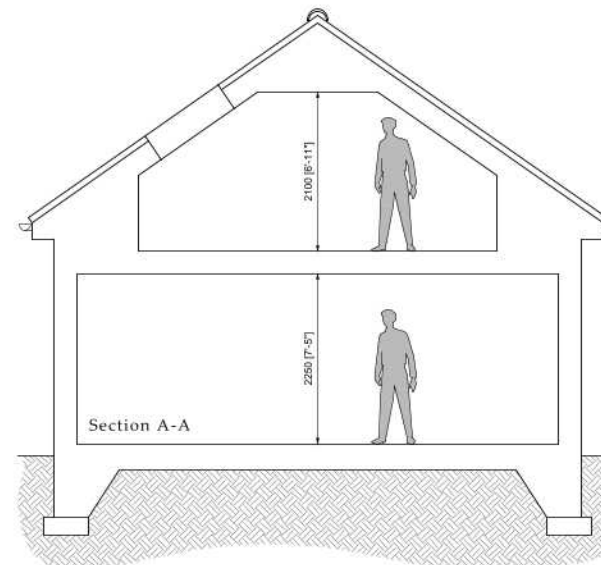
Mezzanine
