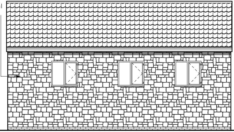
Side Elevation as Proposed.
