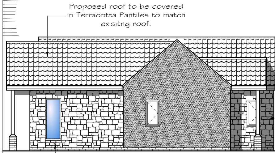
Side Elevation as Proposed.
