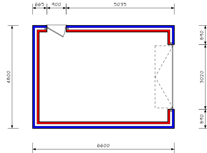
Plan as Proposed.
