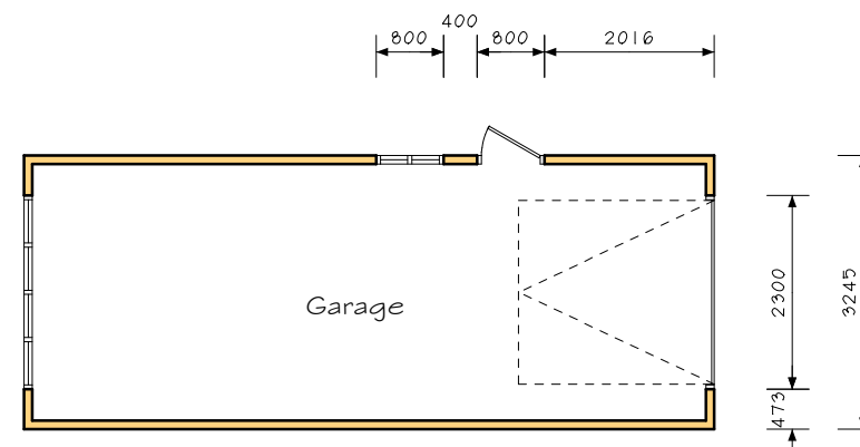
Plan as Existing.
