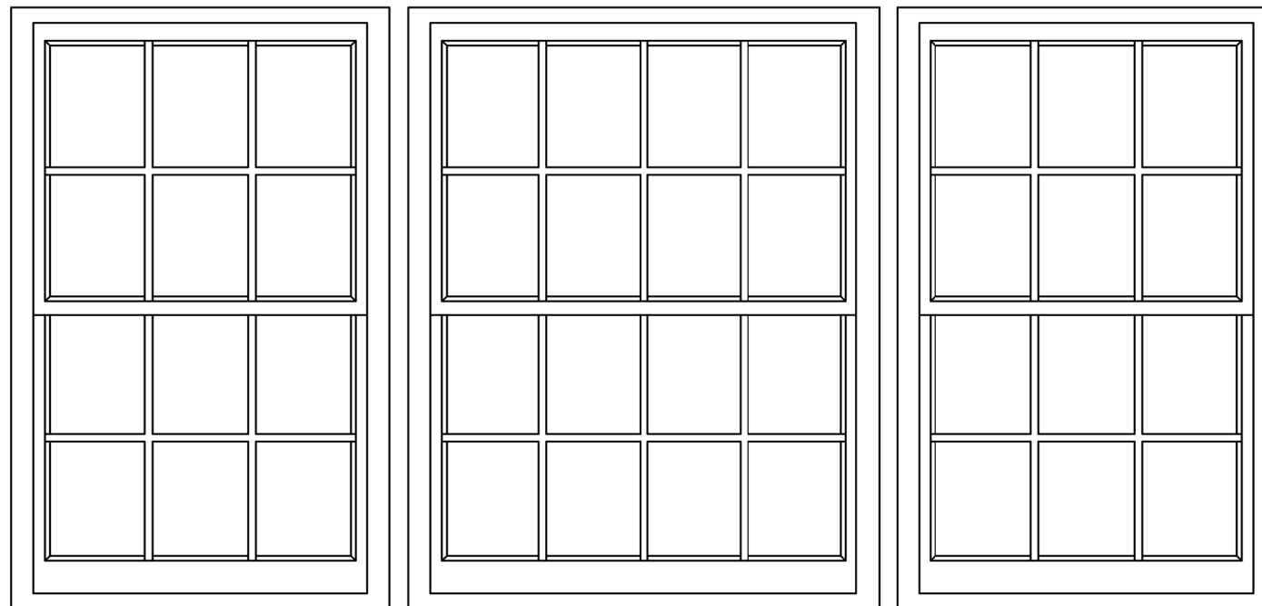
Proposed W1 Front Elevation 1:20 @ A3
