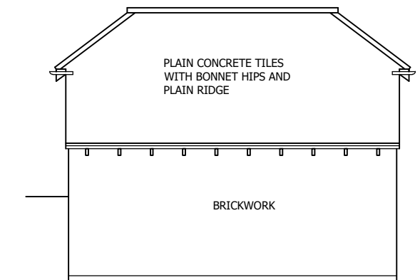
NORTH ELEVATION
