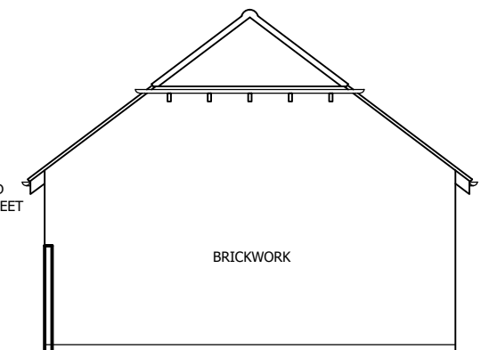
EAST ELEVATION
