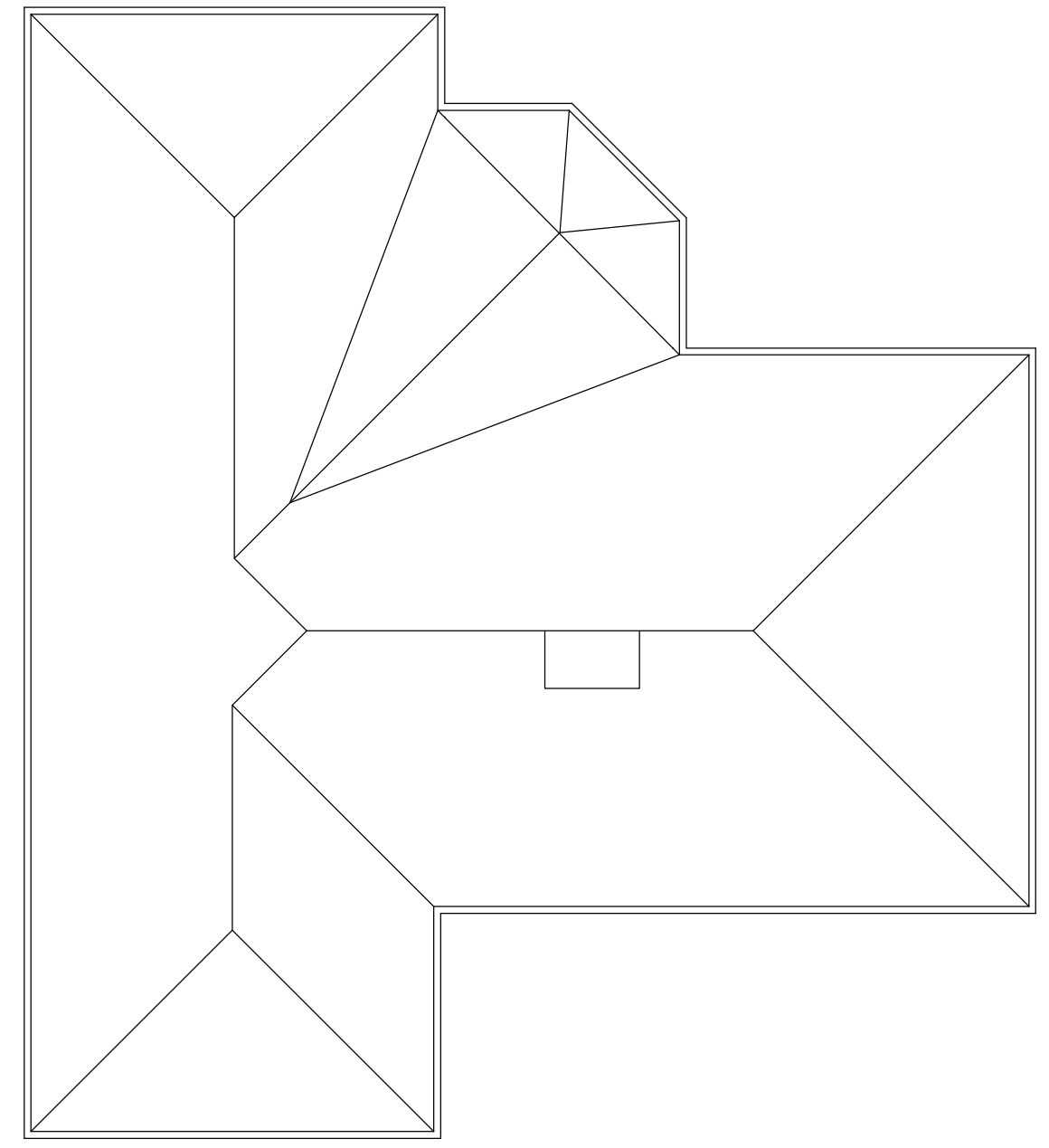
ROOF PLAN
