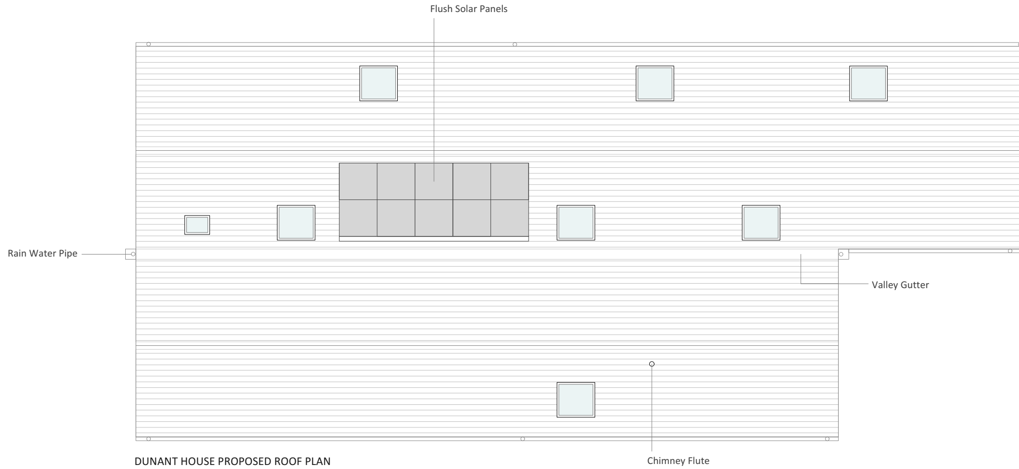
DUNANT HOUSE PROPOSED ROOF PLAN
