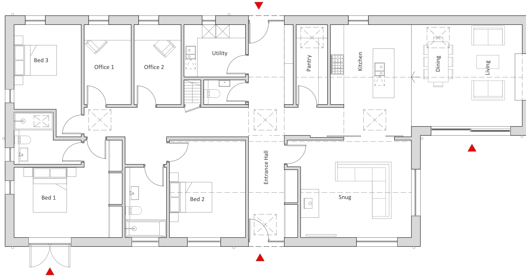
DUNANT HOUSE PROPOSED FLOOR PLAN
