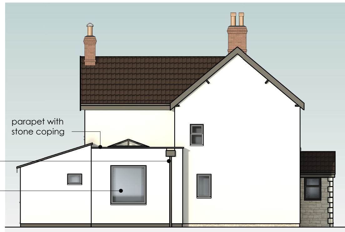
Proposed Side Elevation 2 1 : 100
