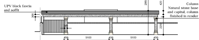
FRONT ELEVATION 1:100 (west elevation)
