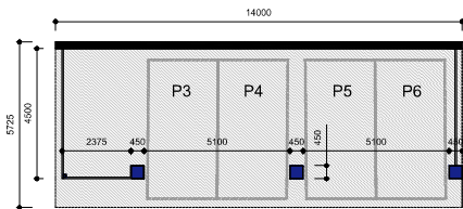
PROPOSED FLOOR PLAN 1:100
