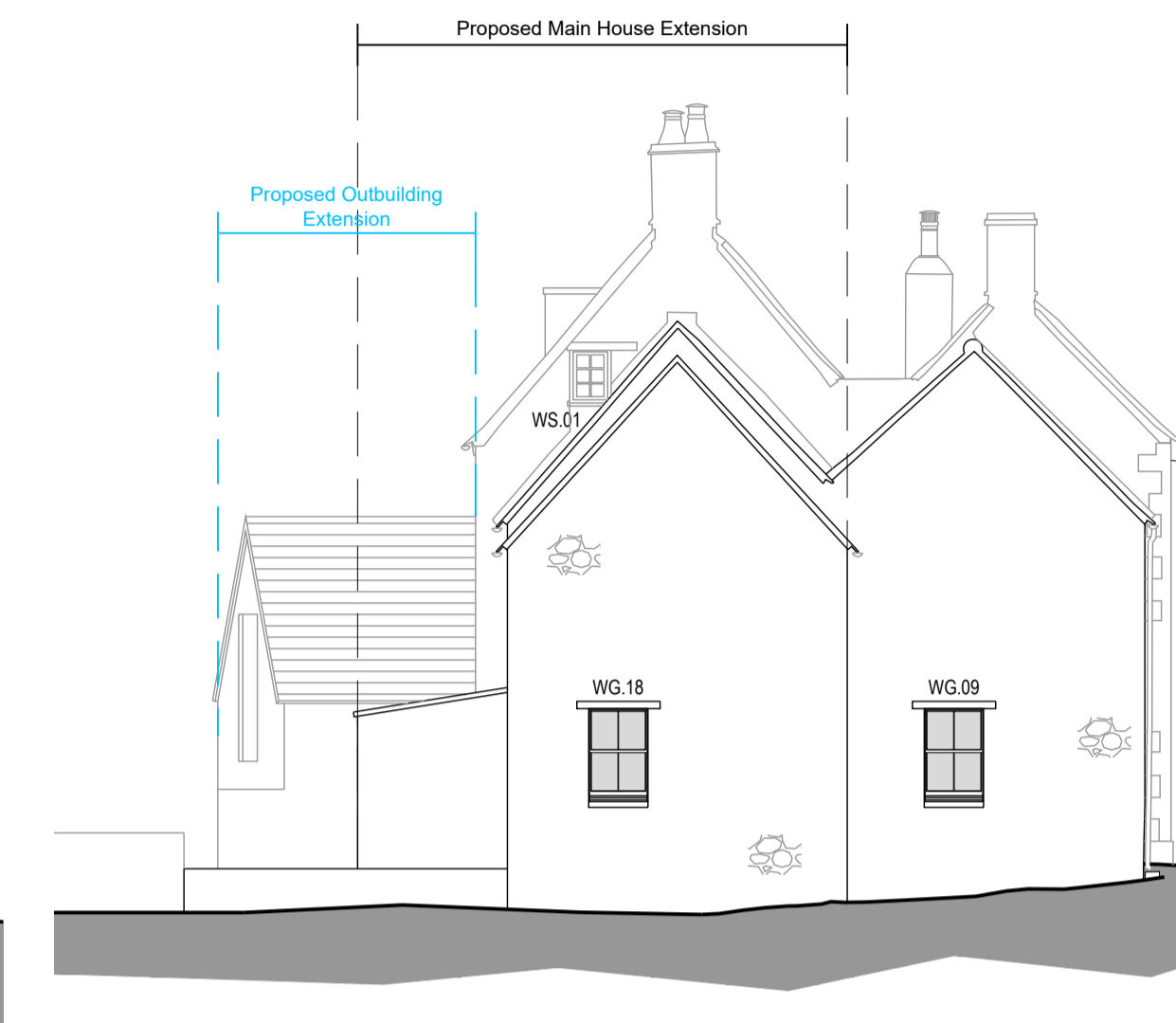
02 East RL200 Elevation
