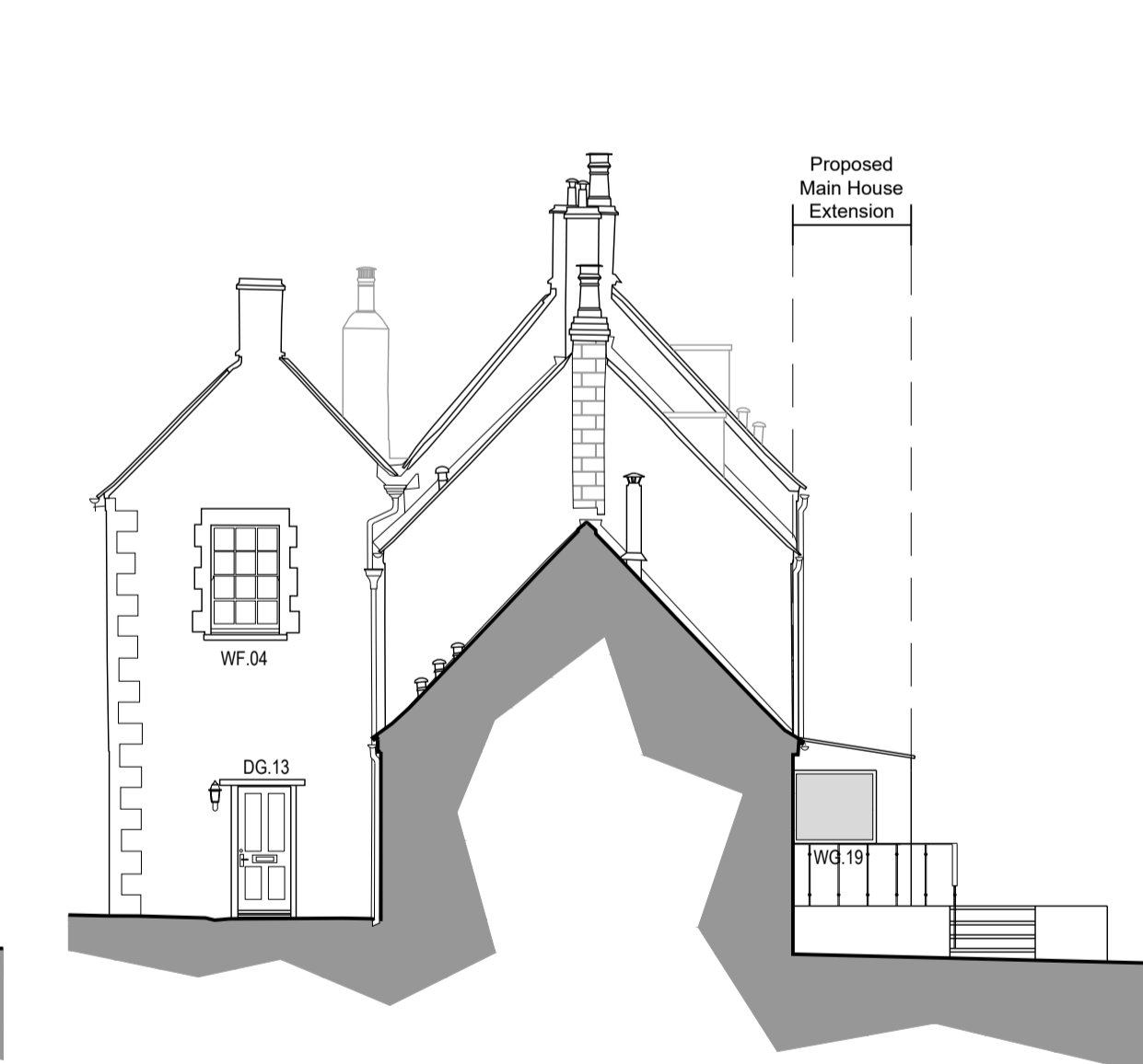
04 West RL200 Elevation
