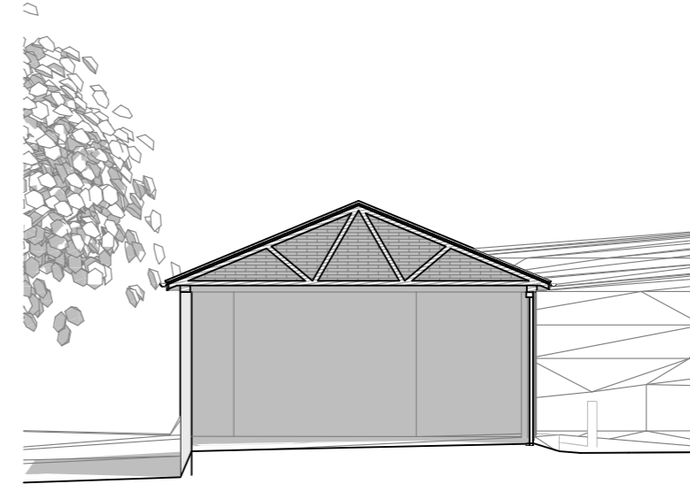
S-02 B-B Building Section B-B Existing 1:100
