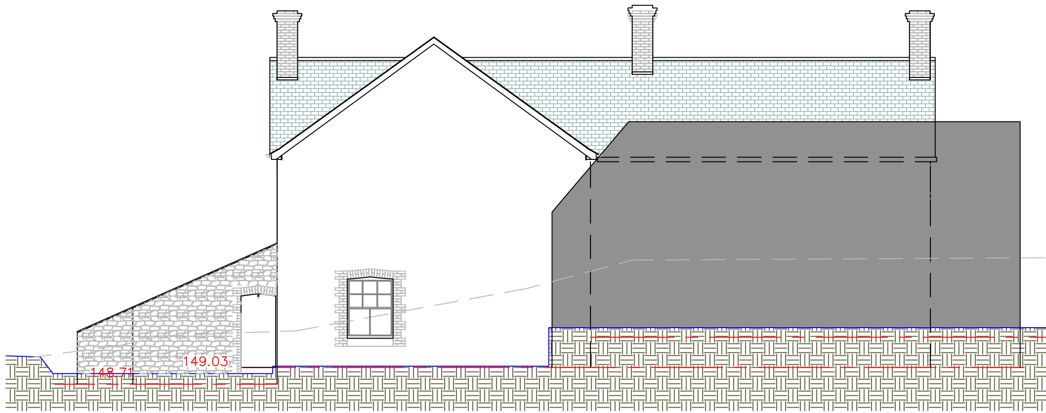
North Elevation 1:100
