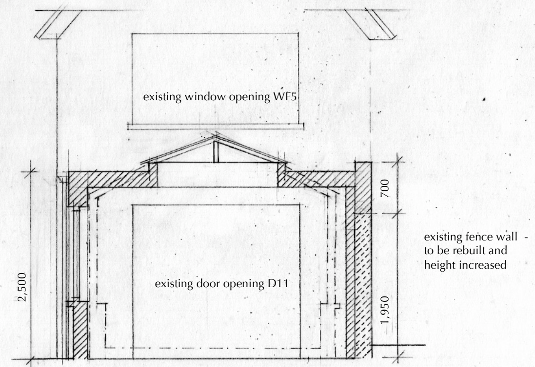
SECTION A THROUGH GARDEN ROOM 1:50
