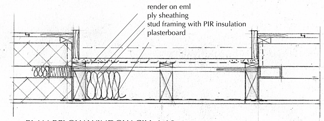
PLAN BELOW WINDOW CILL 1:10
