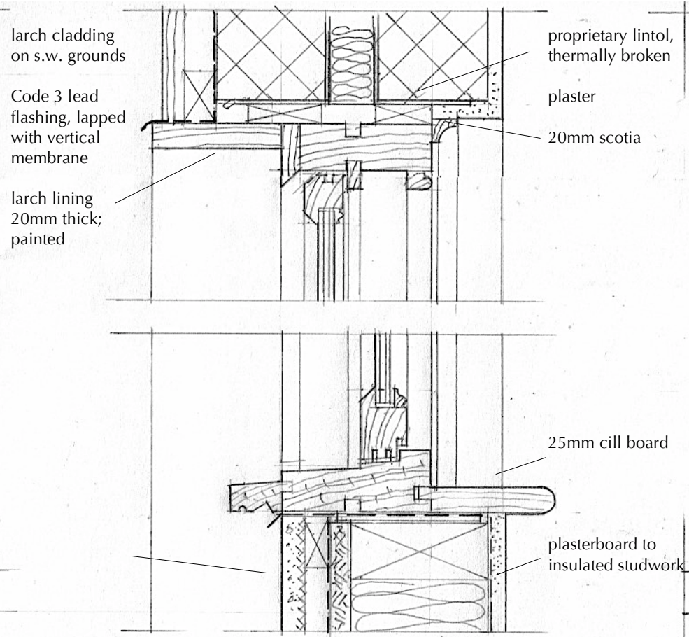
HEAD AND CILL SECTIONS 1:5
