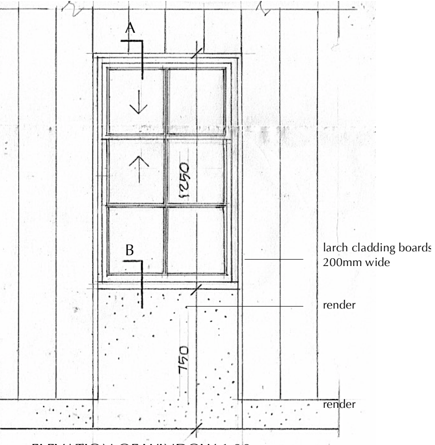
ELEVATION OF WINDOW 1:20
