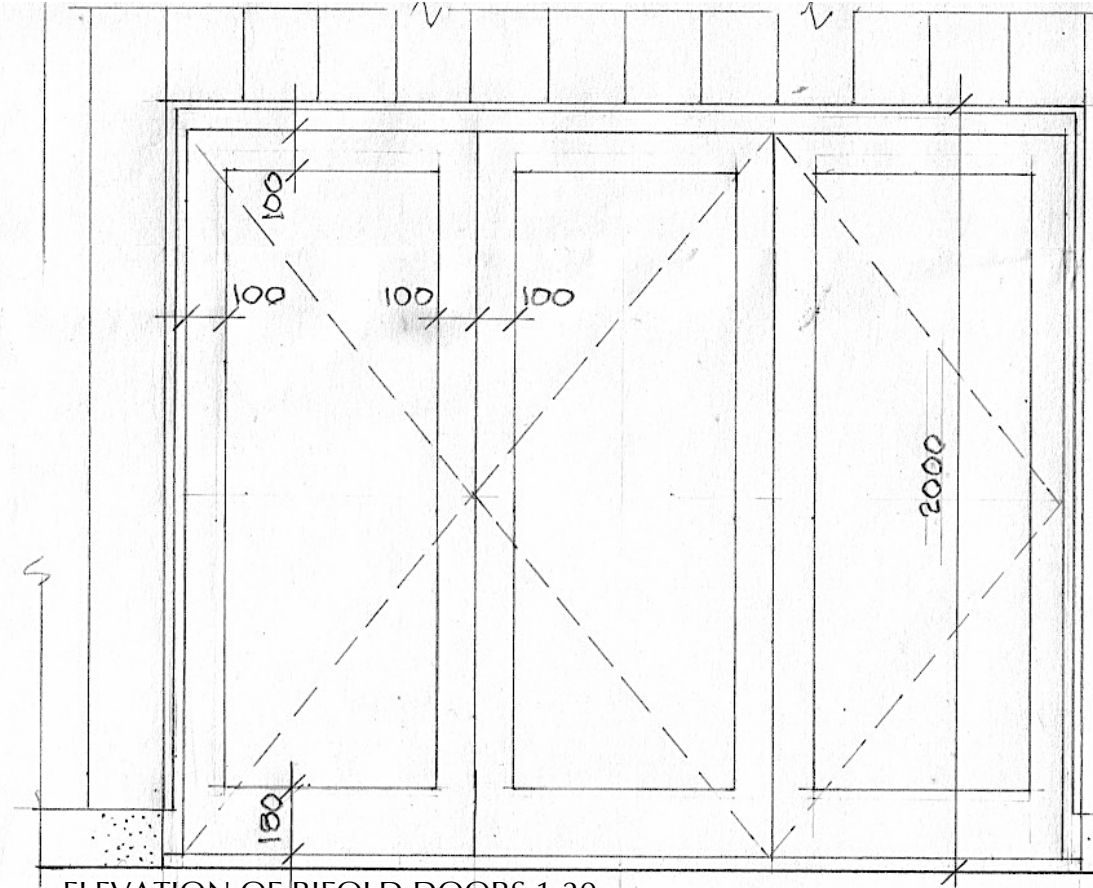
ELEVATION OF BIFOLD DOORS 1:20
