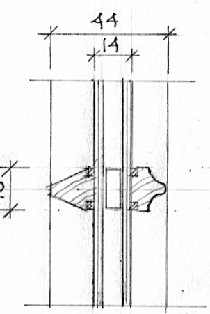
DETAIL OF GLAZING BAR 1:2
