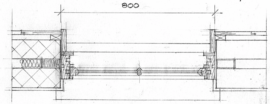
PLAN OF WINDOW ABOVE CILL 1:10
