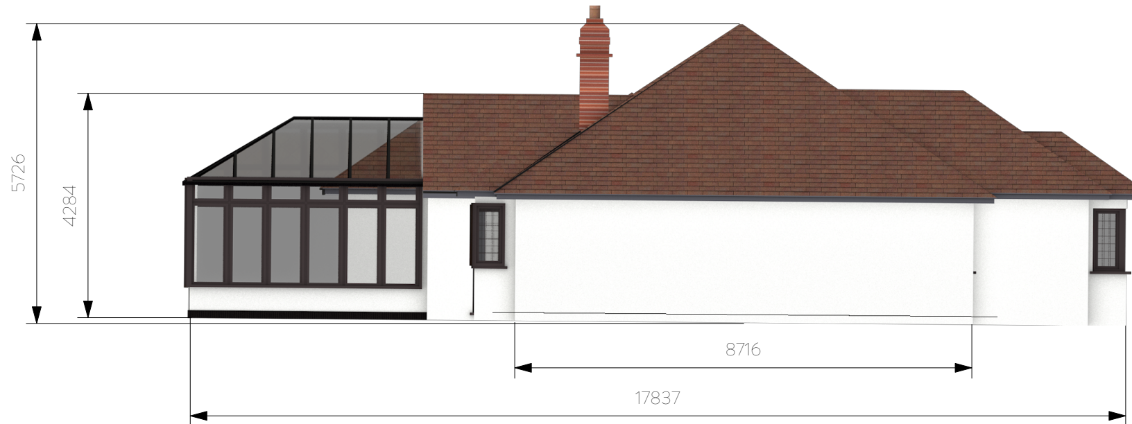
8 EXISTING LEFT SIDE ELEVATION SCALE 1:100
