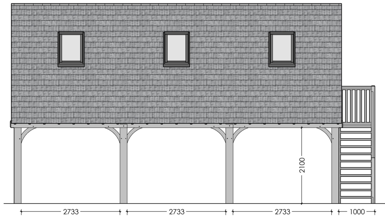
Front Elevation
