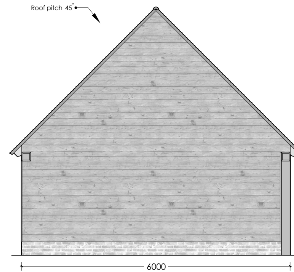
Left Elevation
