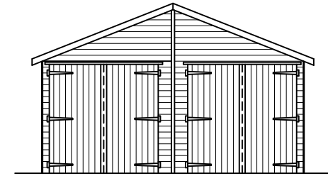
EXISTING FRONT ELEVATION SCALE 1:100
