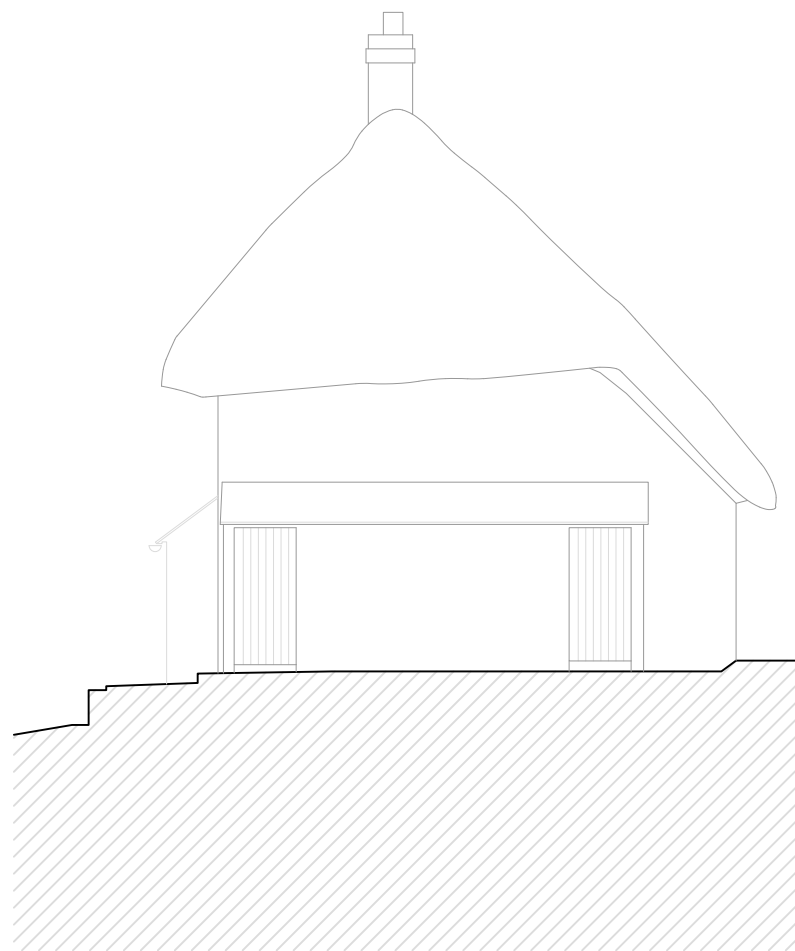
east elevation 1:100 @ a3
