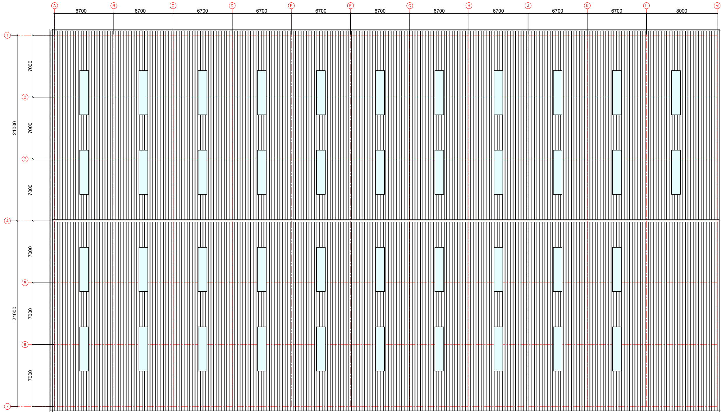
1 Roof Plan Scale: 1:250 (A3)
