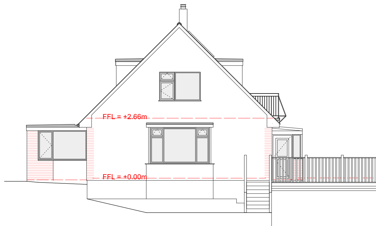
3.0m Datum below FFL South West Elevation
