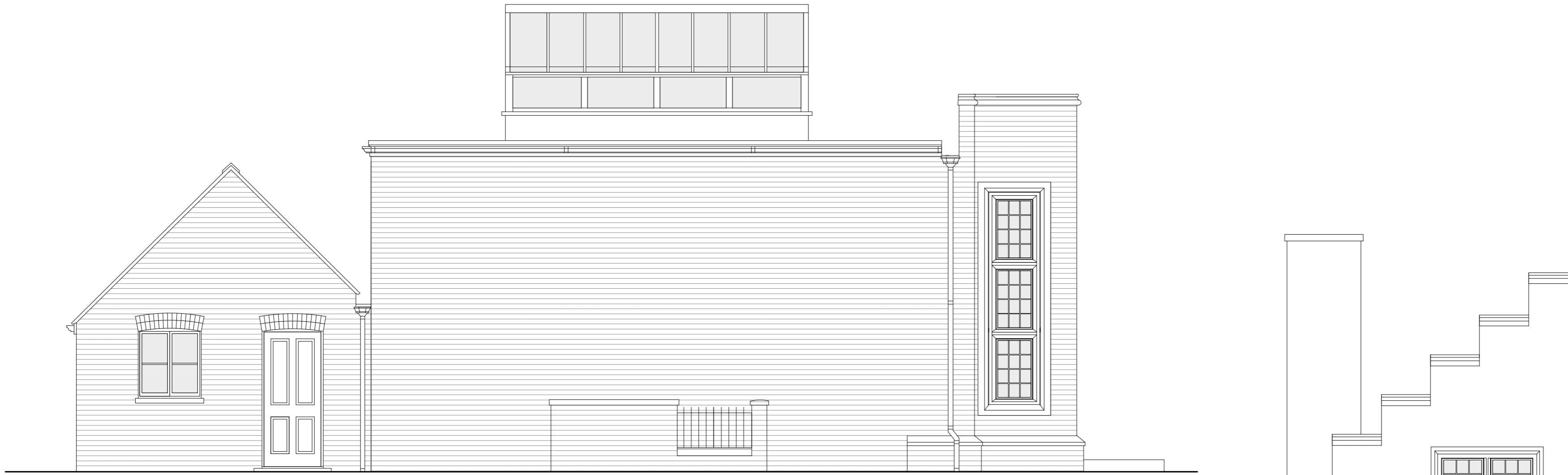
Existing Side Elevation scale 1:50 @ A2
