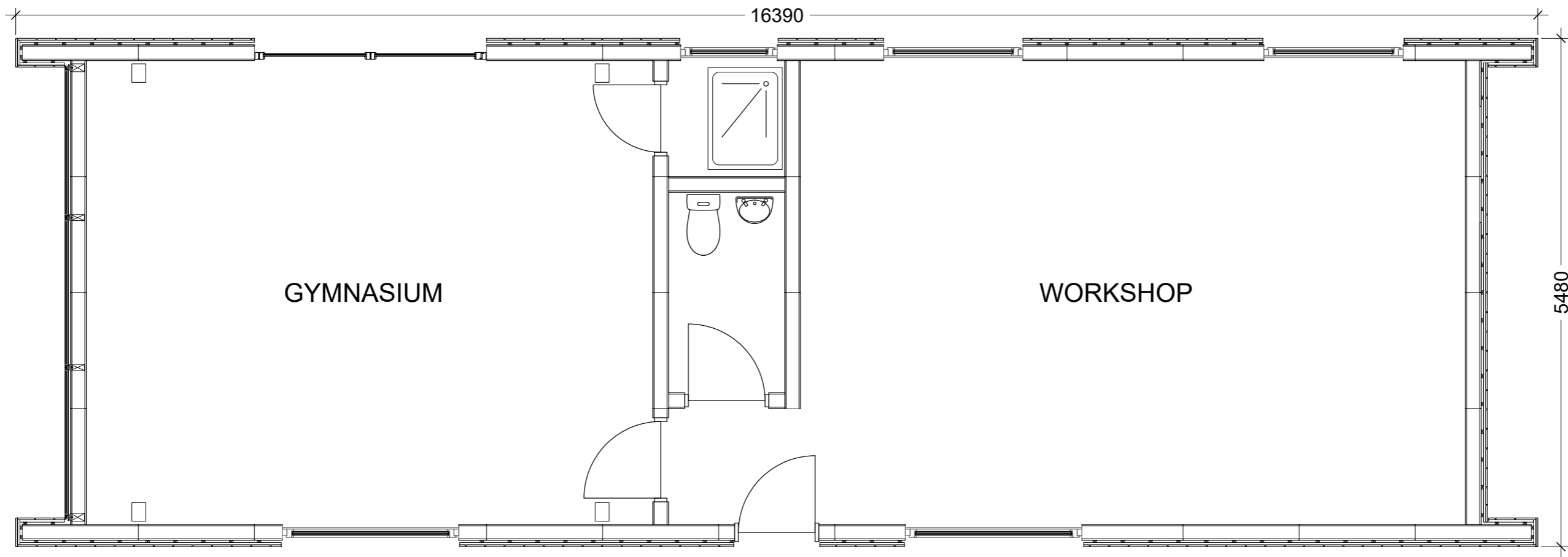
GROUND FLOOR PLAN 1:50
