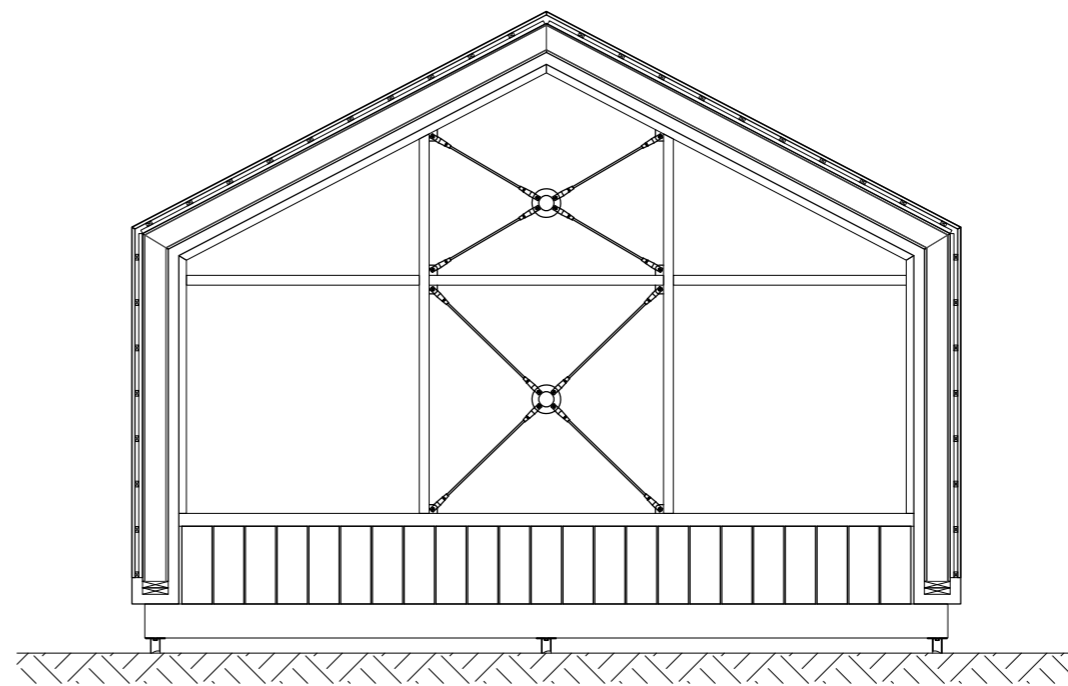
SOUTH ELEVATION 1:50
