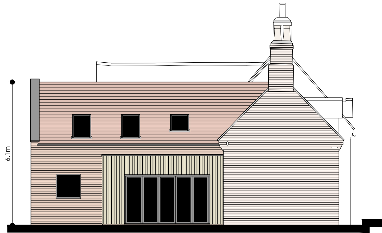
West (Side) Elevation 1:100
