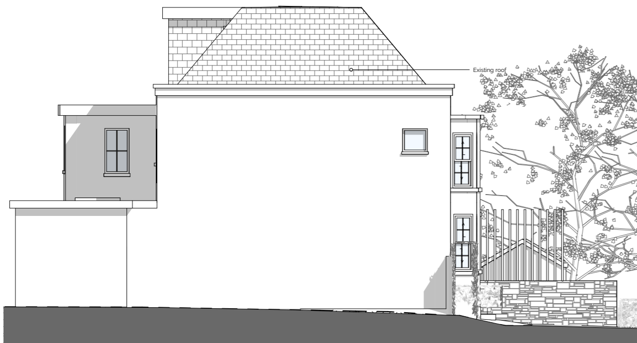
Existing South East Elevation 1:100
