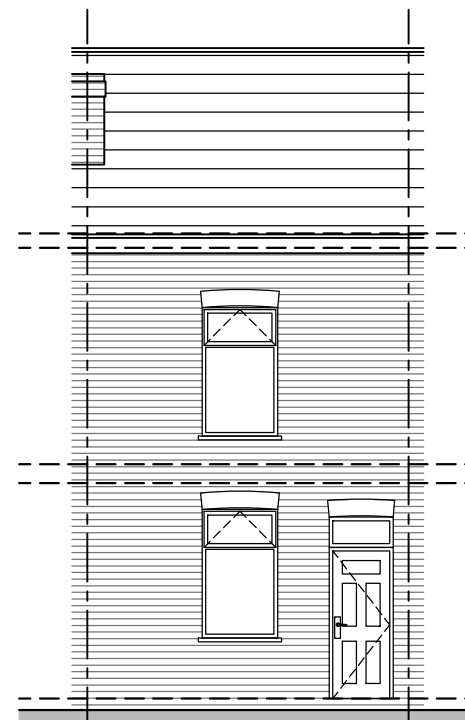
FRONT ELEVATION 1:100
