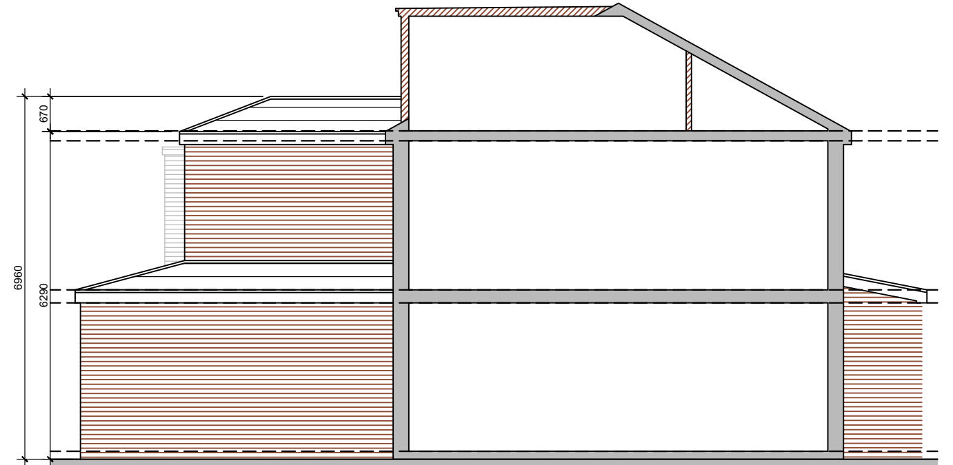
LEFT ELEVATION
