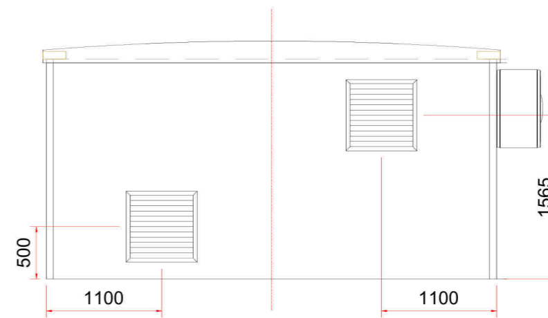
5 Rear Elevation 1:50
