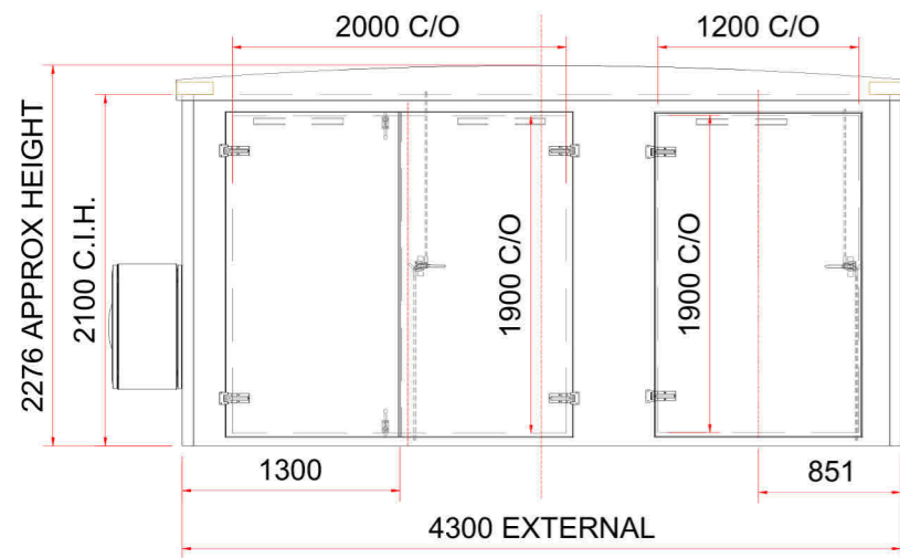
3 Front Elevation 1:50
