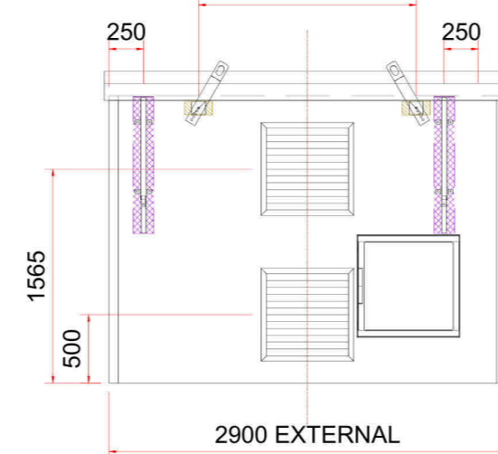
6 Left Elevation 1:50 1592 (LIFTING EYE CENTRES)
