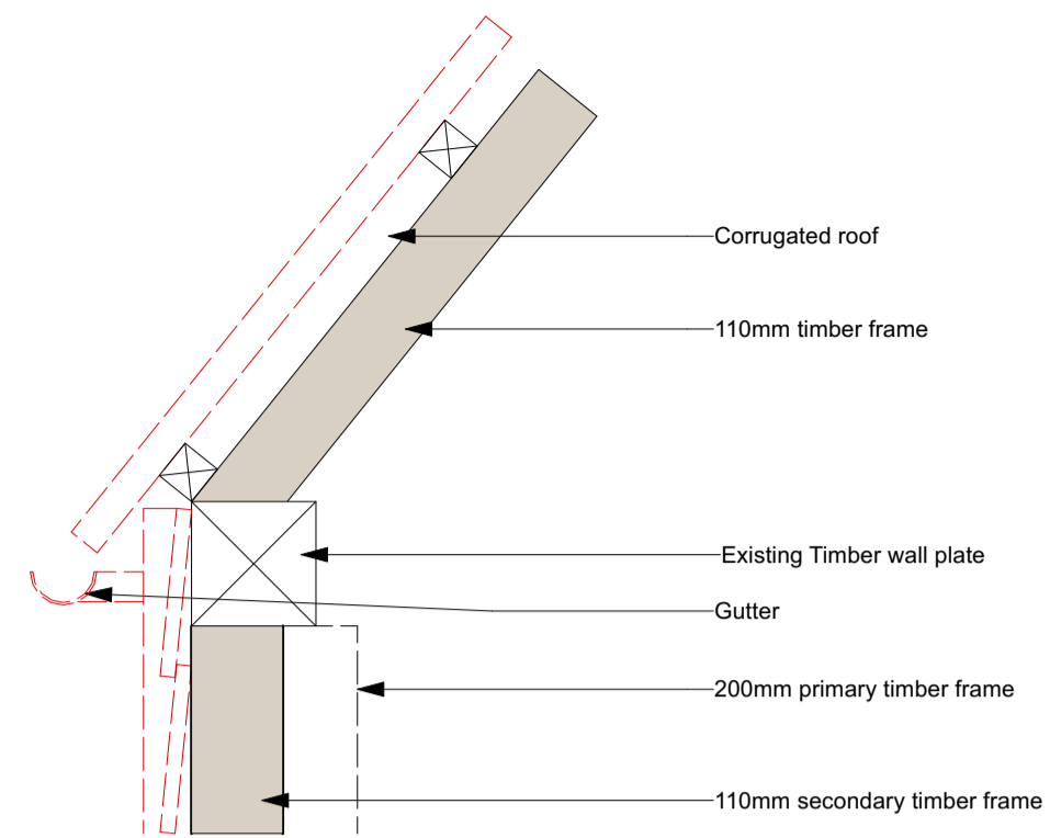
06 | DEMO TYPICAL ROOF/WALL JUNCTION DETAIL (SECTION) 1:10
