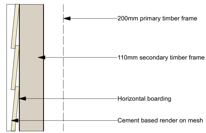
02 | EXISTING TYPICAL WALL DETAIL (SECTION) 1:10
