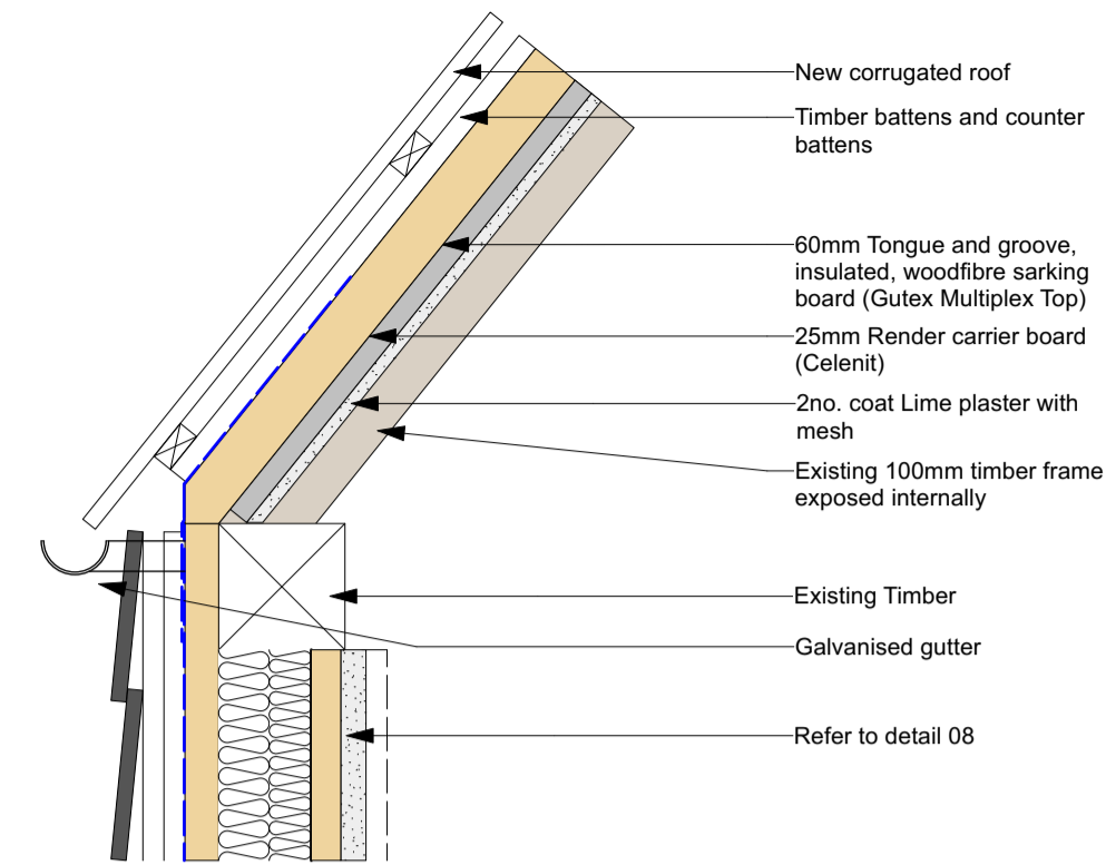
09 | TYPICAL ROOF/WALL JUNCTION DETAIL (SECTION) 1:10
