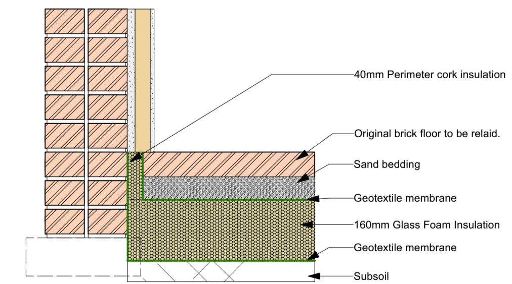
10 | TYPICAL FLOOR/WALL JUNCTION DETAIL - BRICK (SECTION) 1:10
