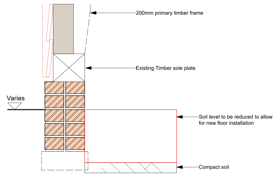
04 | DEMO TYPICAL FLOOR/WALL JUNCTION DETAIL (SECTION) 1:10
