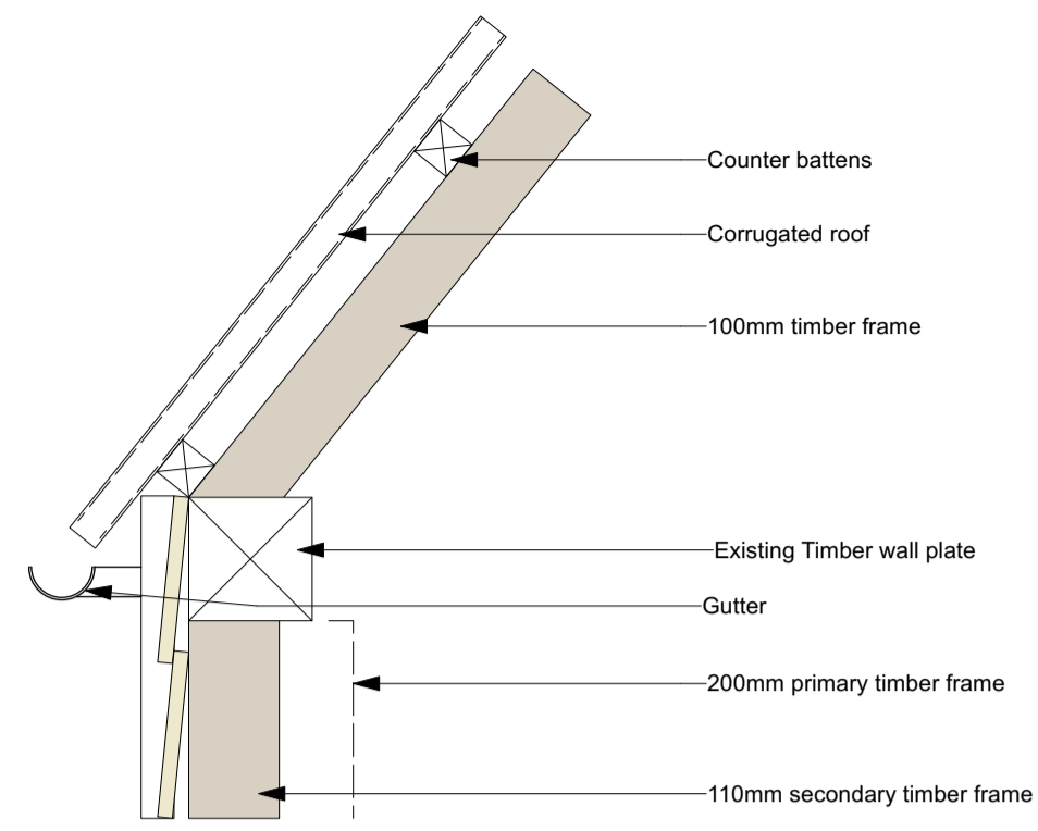
03 | EXISTING TYPICAL ROOF/WALL JUNCTION DETAIL (SECTION) 1:10
