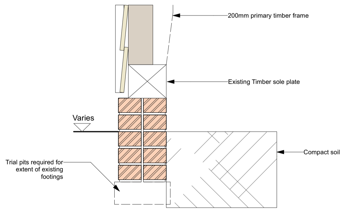
01 | EXISTING TYPICAL FLOOR/WALL JUNCTION DETAIL (SECTION) 1:10
