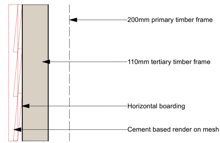
05 | DEMO TYPICAL WALL DETAIL (SECTION) 1:10
