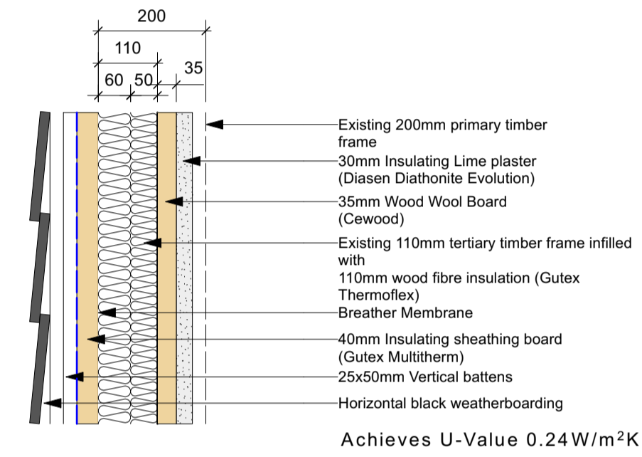
08 | TYPICAL WALL DETAIL (SECTION) 1:10
