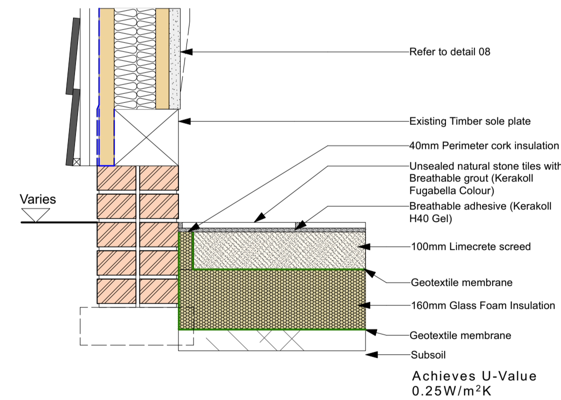
07 | TYPICAL FLOOR/WALL JUNCTION DETAIL - SCREED (SECTION) 1:10
