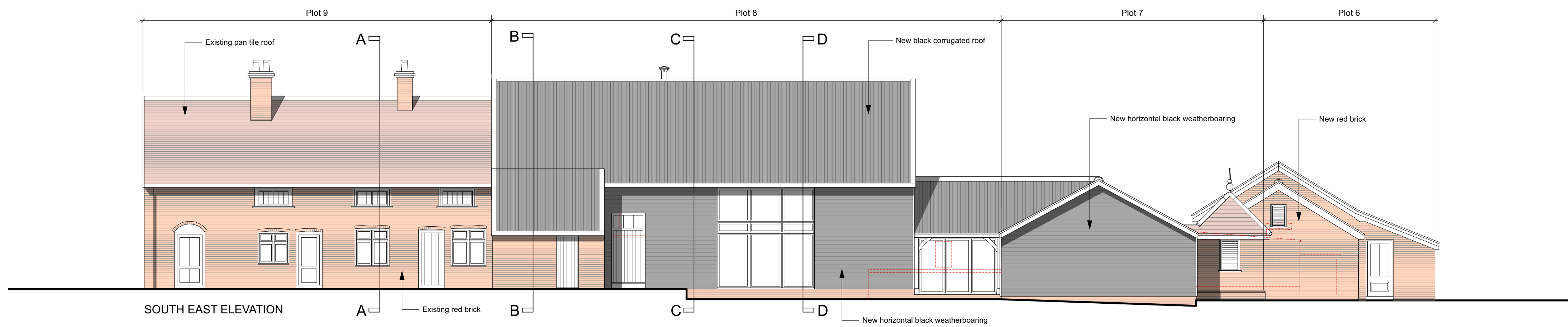
Building 2 Proposed Elevations Scale: 1:100
