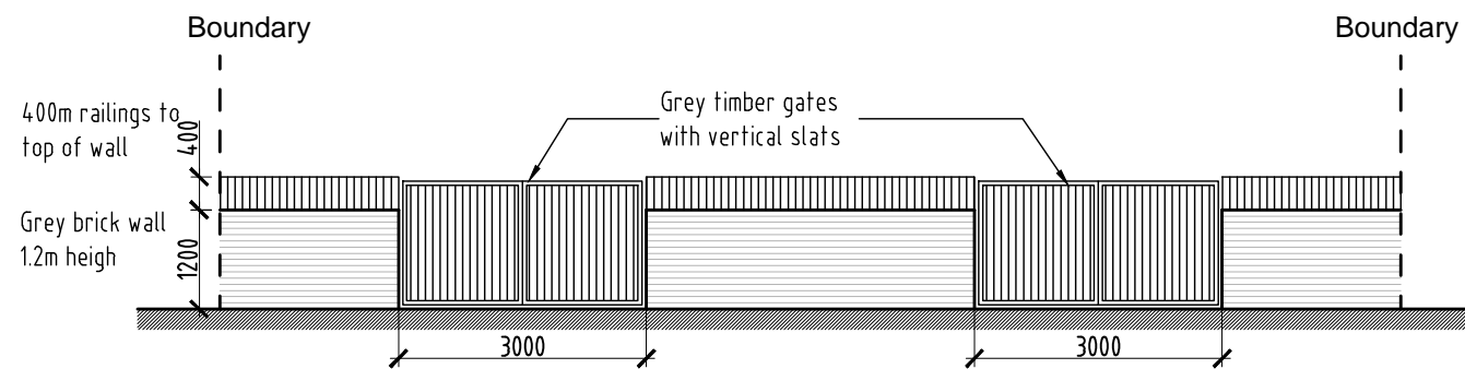
Front Elevation Facing Parkwood Road (Boundary sides the same) 1:100
