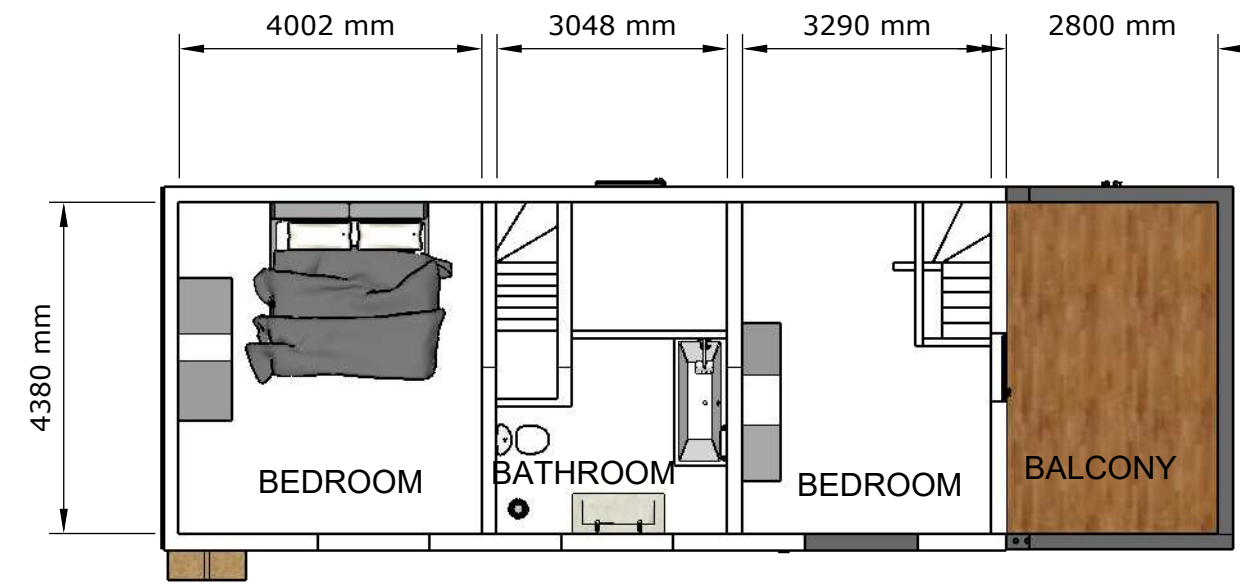
FIRST FLOOR
