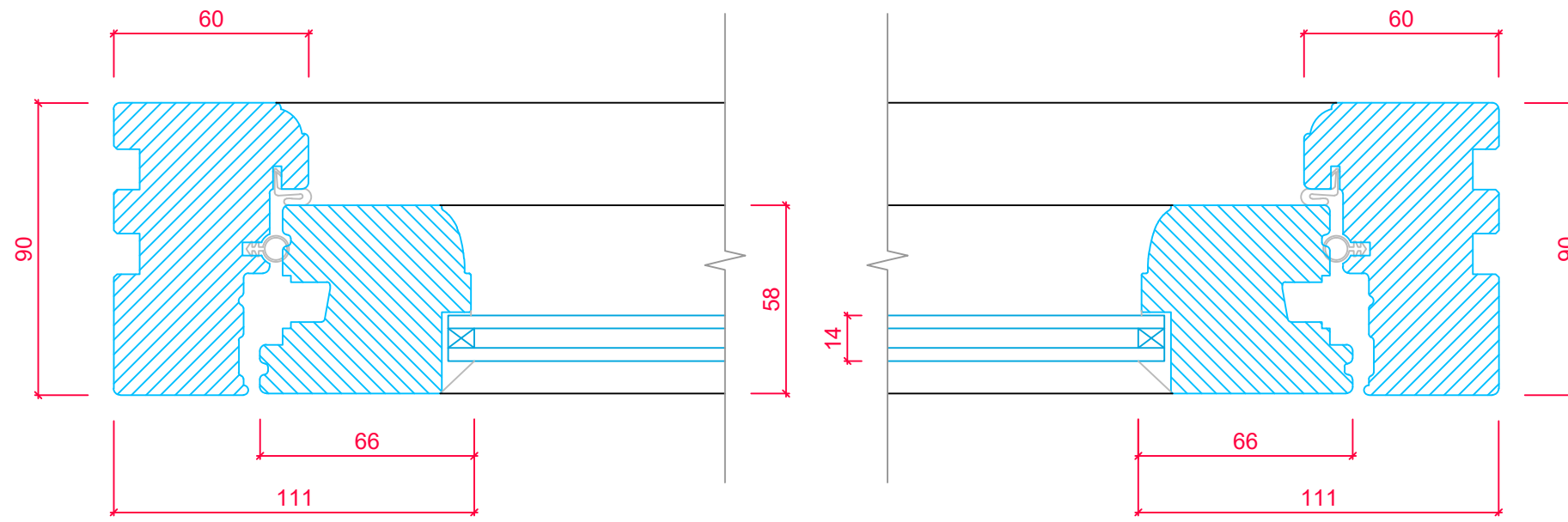
CASEMENT CROSS SECTION 'A-A'
