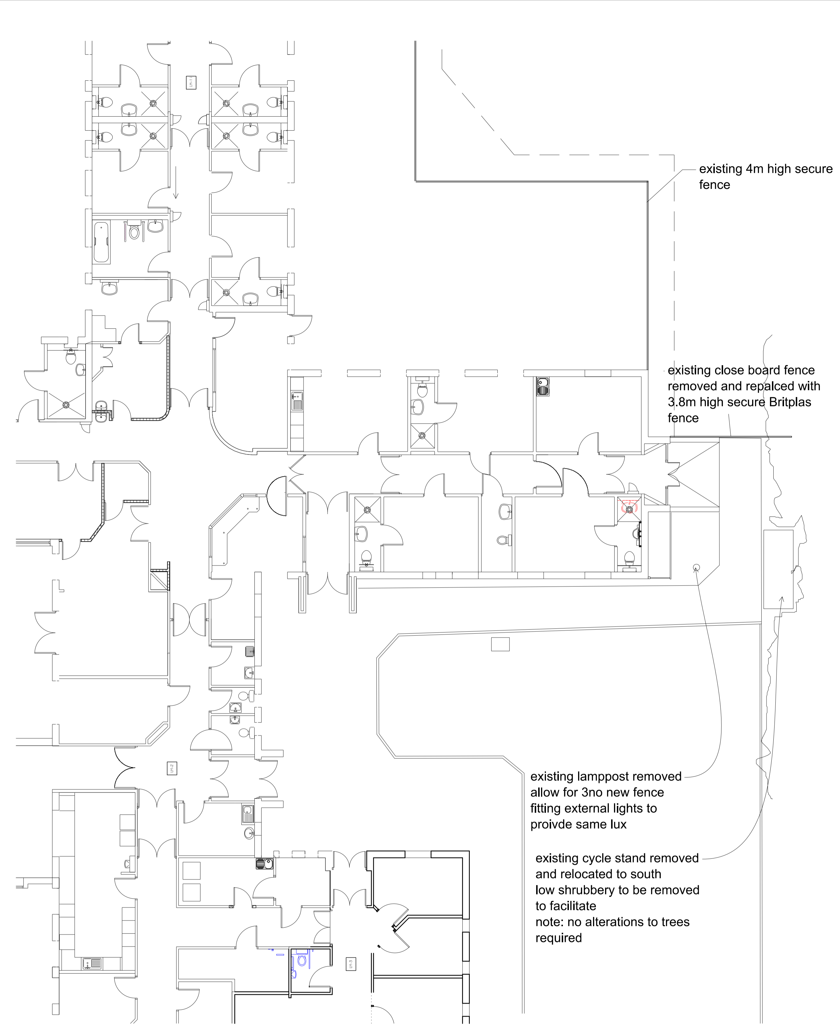
Existing Plan - new secure fence to 136 unit
