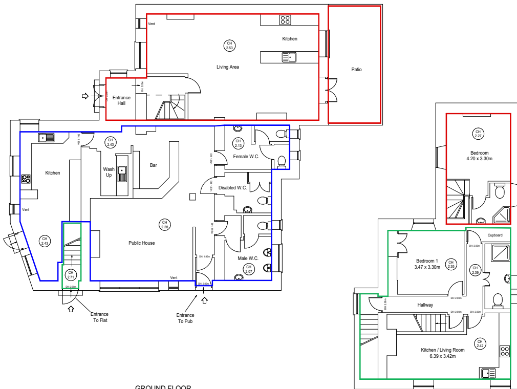
GROUND FLOOR Approx Gross Internal Area: 159.6 m 2 - 1,718 ft 2
