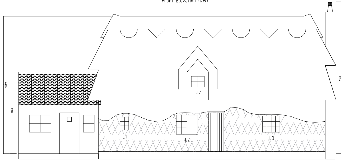
Front Elevation (NW)
