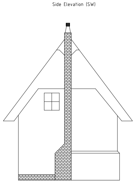
Side Elevation (SW)
