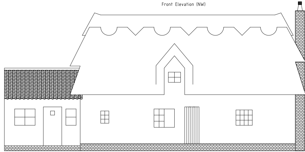
Front Elevation (NW)
