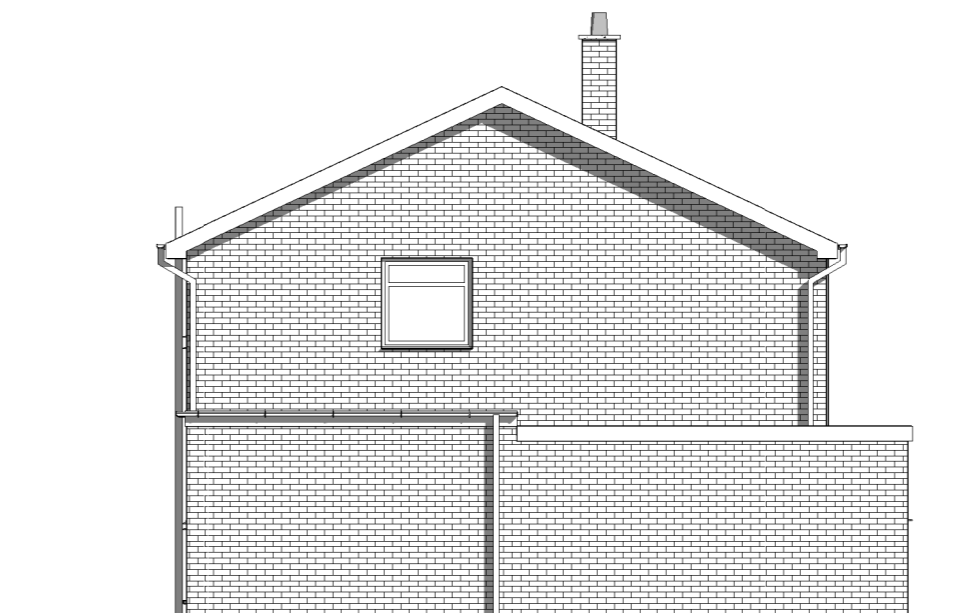
Existing Side Elevation 2 1 : 100 East
