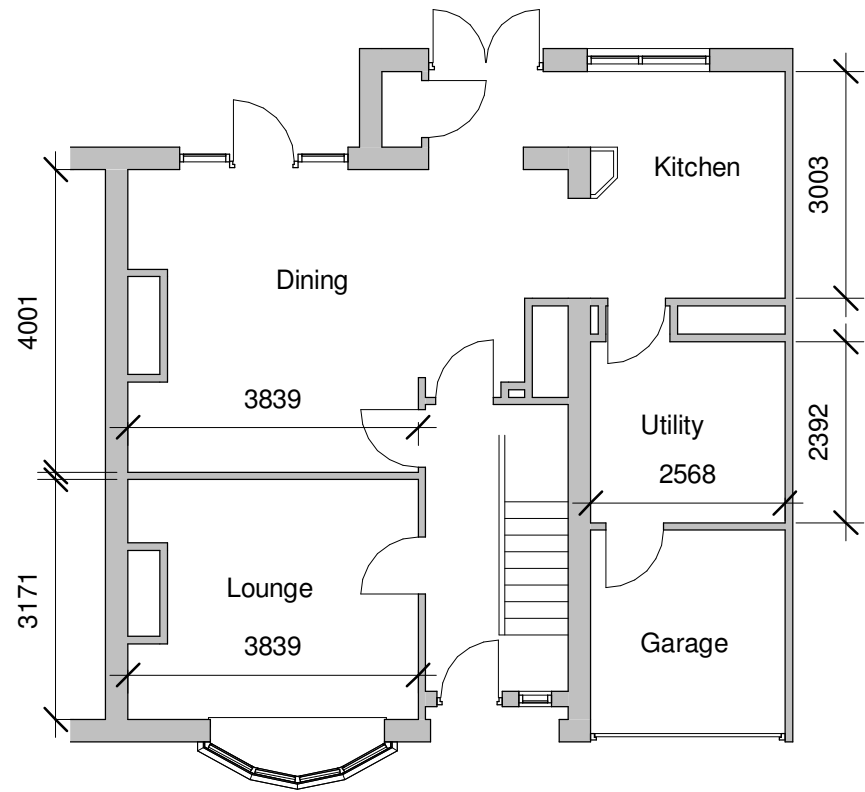
Ground 1 : 100
