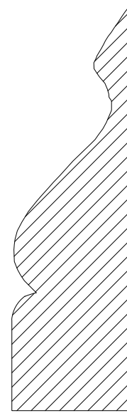
Proposed Living/Kitchen Architrave Detail (1:1)
