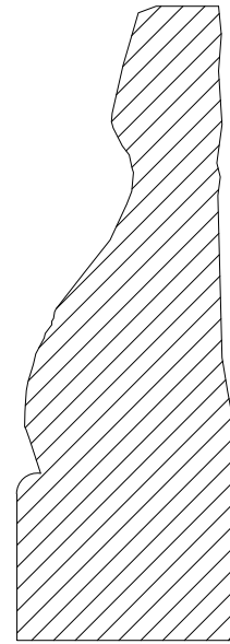
Existing Living/Kitchen Architrave Detail (1:1)
