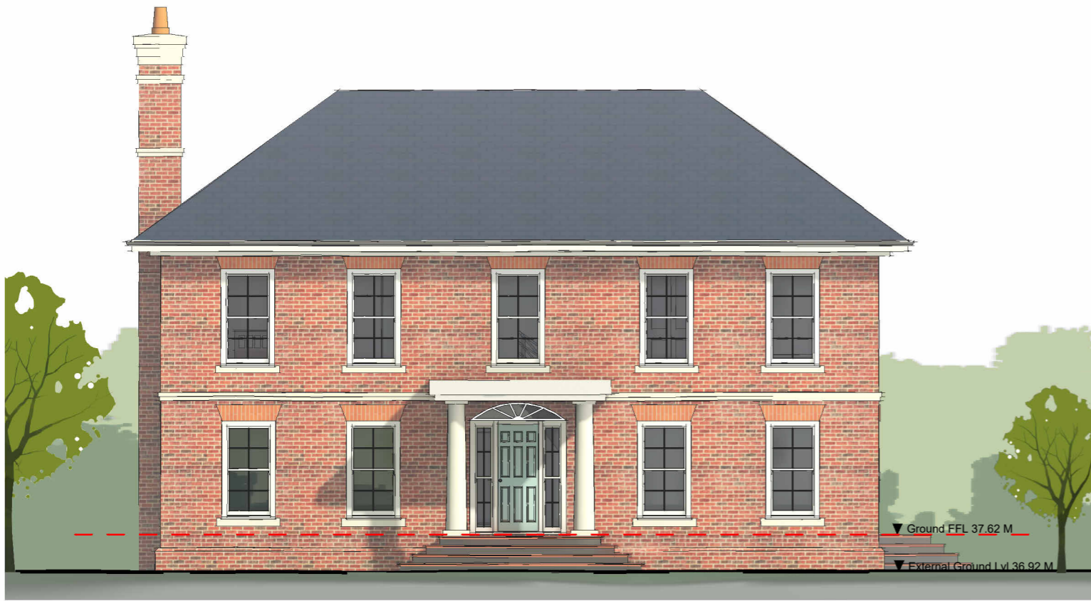
Front-East 1 : 100
