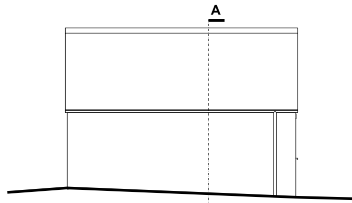
NORTHWEST ELEVATION scale @ 1:100
