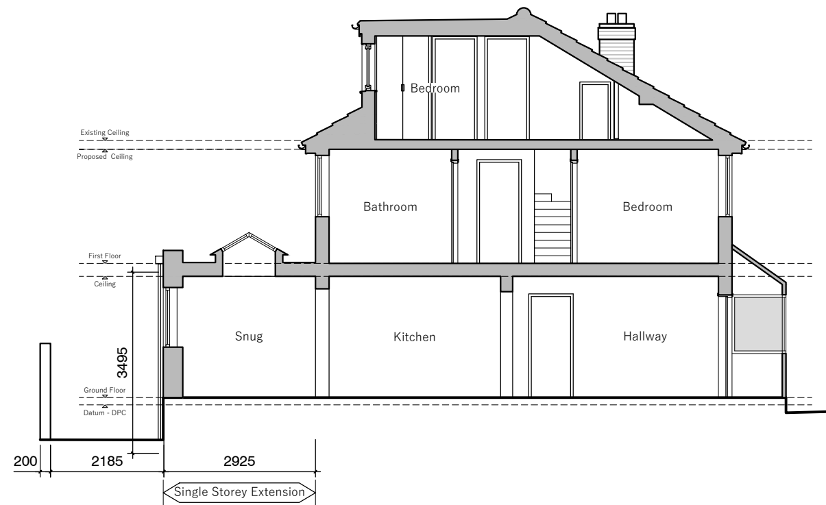
Proposed - Section A2
