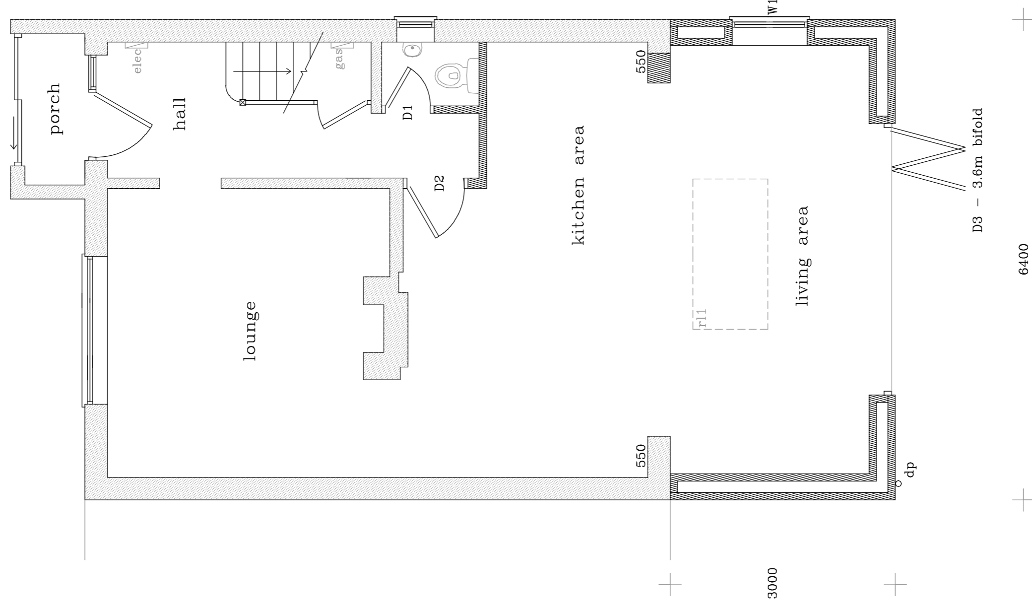
GROUND FLOOR
